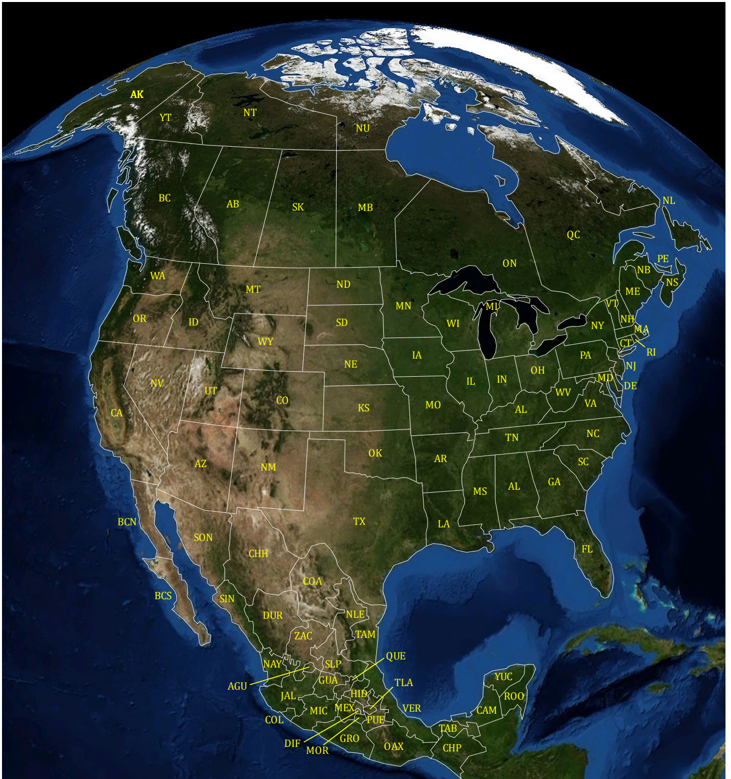
Figure 1. States and provinces plotted on an enhanced satellite image of North America from space. See Table 1 for a key to abbreviated place names. The background image, based on an observer directly over Texas, shows ground cover in the month of July. The background image was generated with the NASA World Wind 1.4 mapping tool ( http://worldwind.arc.nasa.gov/download.html ).
